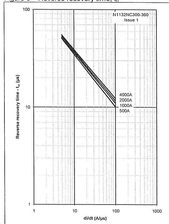
Figure 8 – Reverse recovery time, t_{rr}
