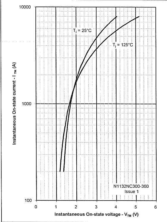
Figure 1 - On-state characteristics of Limit device
