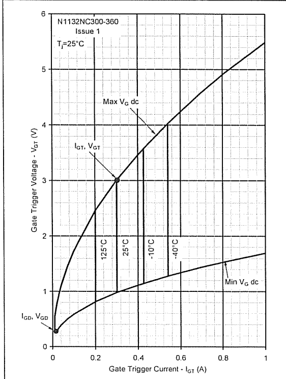
Figure 3 - Gate Characteristics - Trigger Limits
