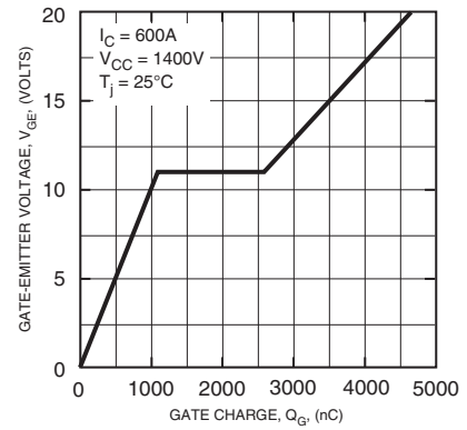
GATE CHARGE VS. V_GE
